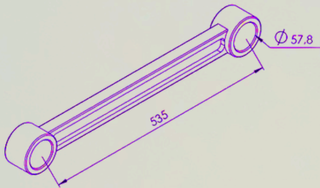
MSU1015 TENSOR FIJO 535MM MB SUSPENSYS
