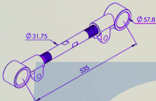
MSU1014 TENSOR REGULABLE 535MM MB SUSPENSYS
